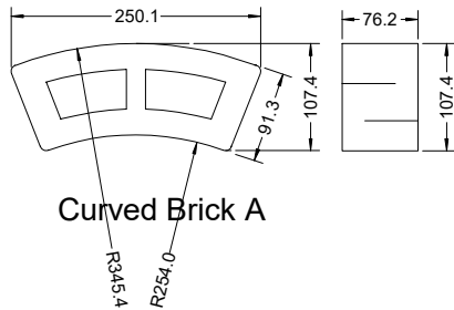
"Select" Brick With Holes
