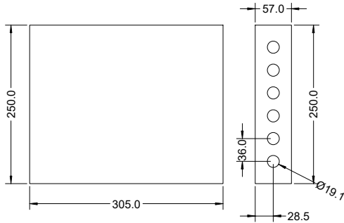
Perforated Clay Tile
