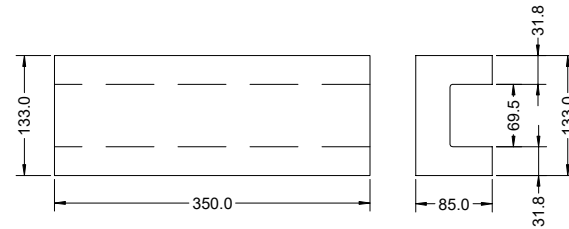
Clay Chimney Connector
