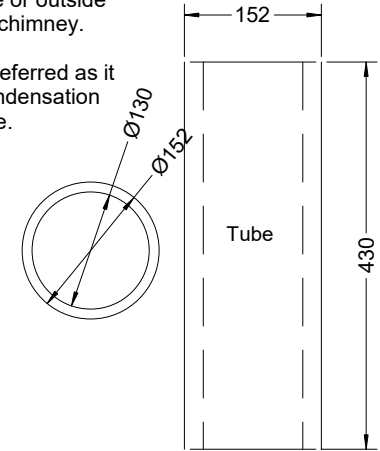
Clay Chimney Connector
